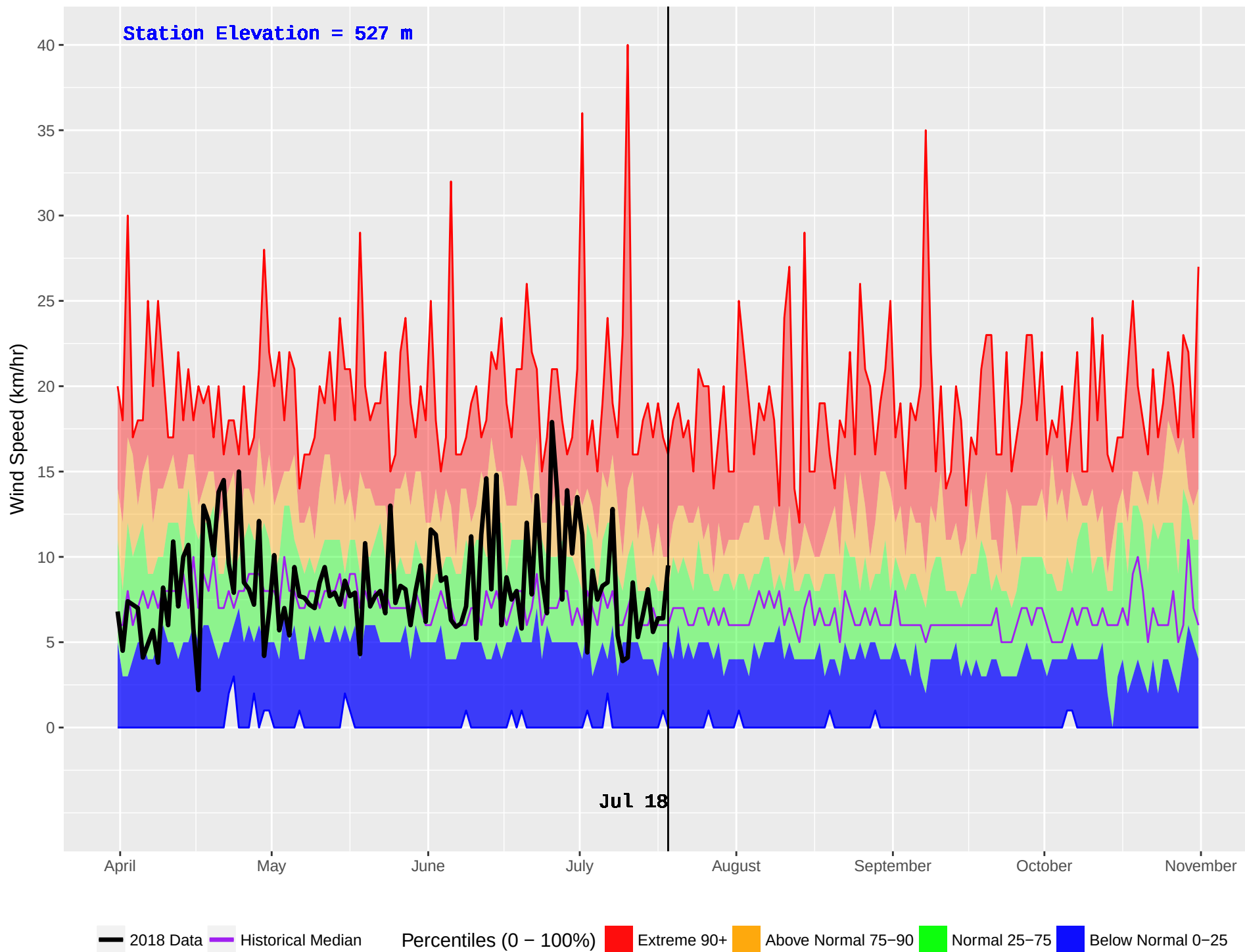
SALMON ARM (346) : Historical (1976–2016) and Current (2018) Daily Wind Speed
