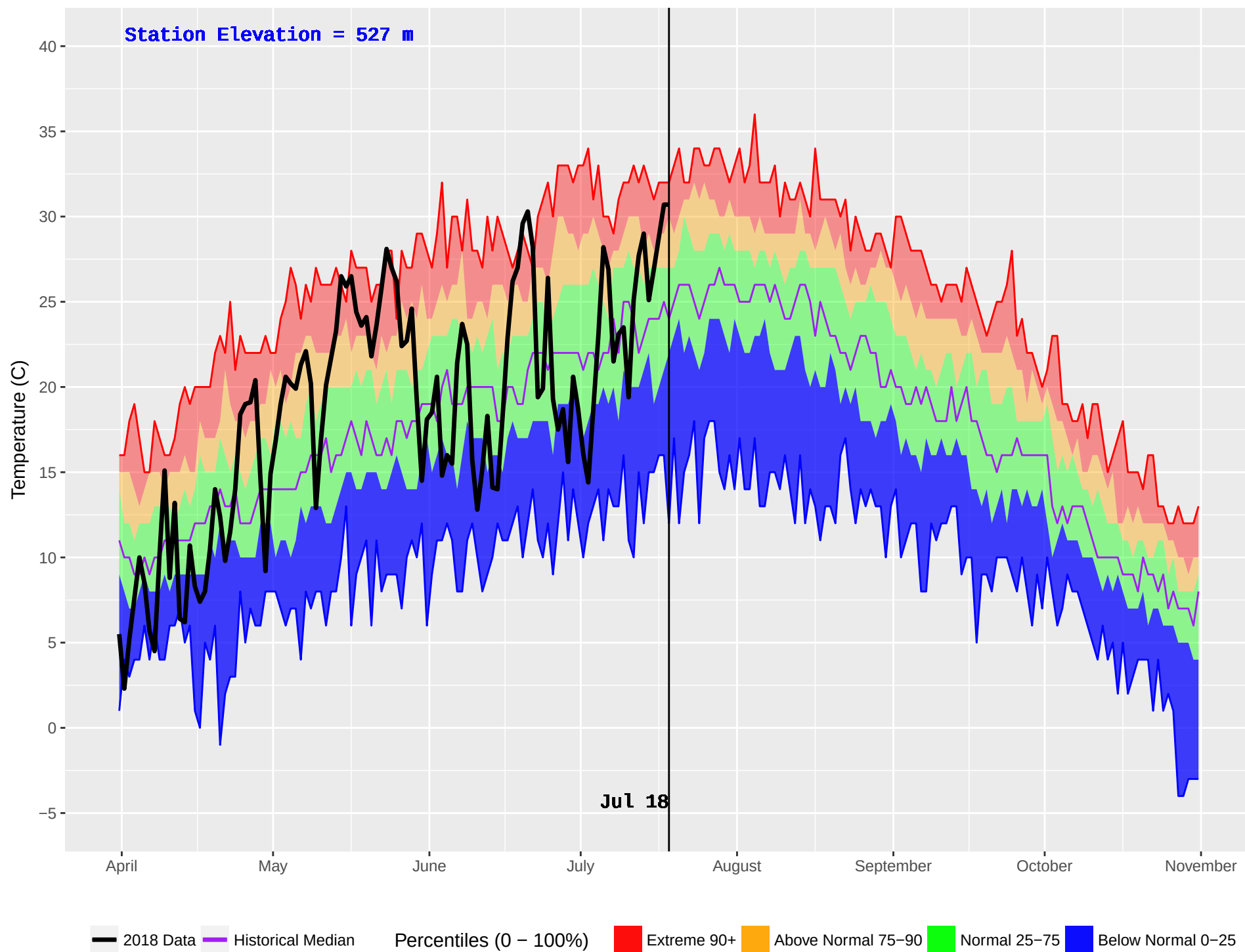
SALMON ARM (346) : Historical (1976–2016) and Current (2018) Daily Temperature
