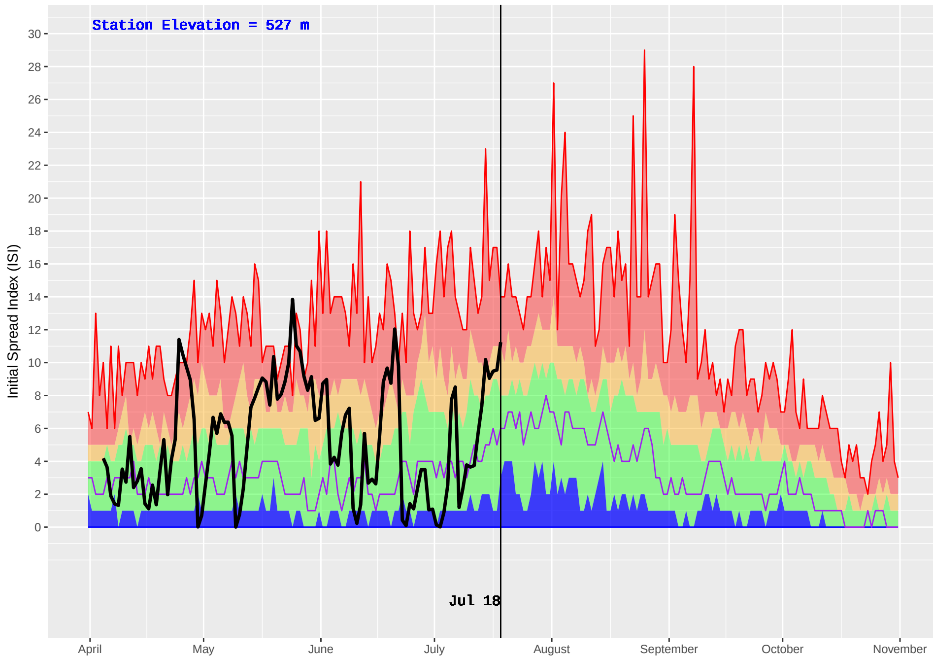
SALMON ARM (346) : Historical (1976–2016) and Current (2018) Daily Initial Spread Index (ISI)
