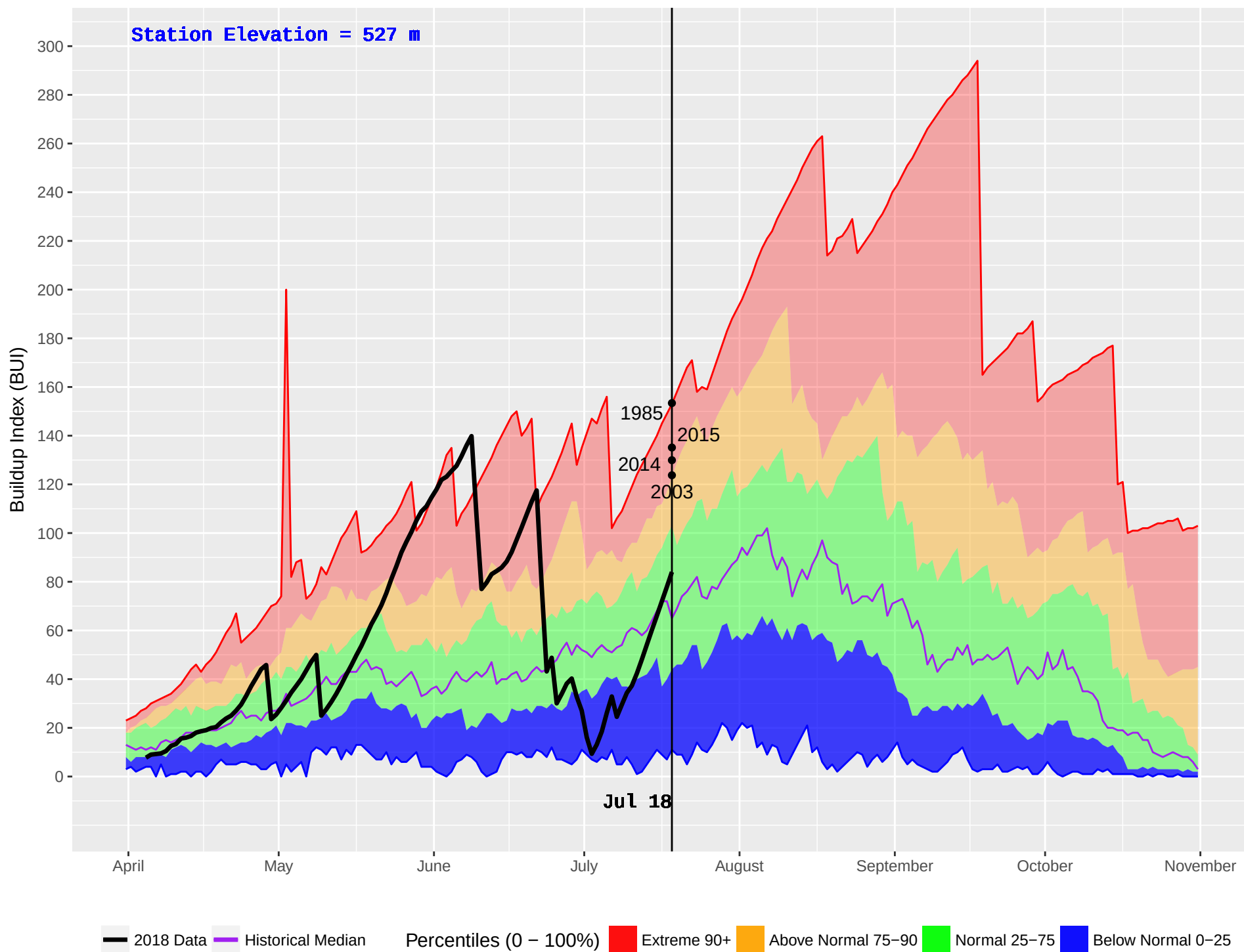
SALMON ARM (346) : Historical (1976–2016) and Current (2018) Daily Buildup Index (BUI)
